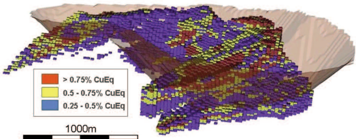
Santo Domingo copper equivalent block model with superimposed pit outline (not optimized and not NI 43-101 compliant)
